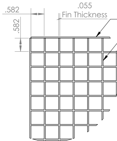
DETAIL B SCALE 1 : 2
